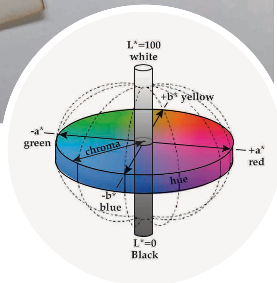
Illustration of CIE LAB L^*a^*b^* color space. Color is measured along three spectrums – L (black to white), a (green to red), and b (blue to yellow) and recorded as a set of three values. Higher L values and lower a and b values correspond to lighter colors.
